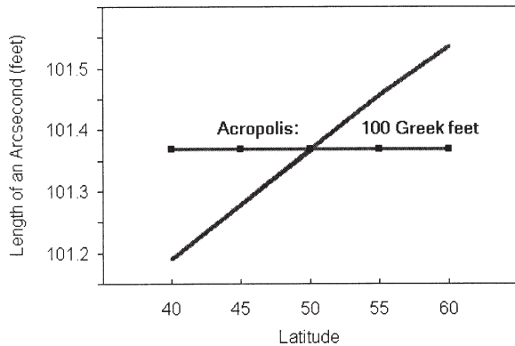
Figure 1. Arcsecond of Great Circle.
