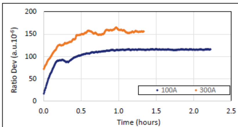
Figure 1. Measured values of a 0.001 \Omega resistive shunt at 100 A (blue curve) and 300 A (orange curve) vs a 1 \Omega standard resistor. The measurement setup and environmental condition are equivalent in both measurements.
