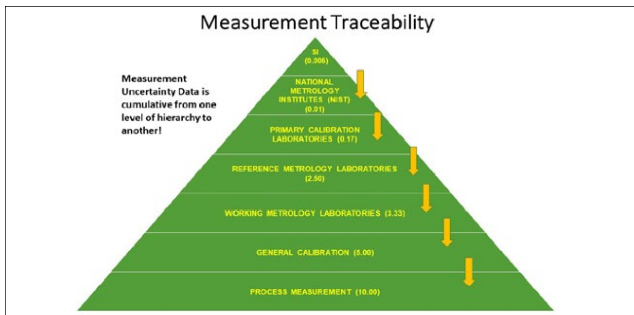
Figure 6. Measurement Traceability Pyramid Used with Measurement Uncertainty
