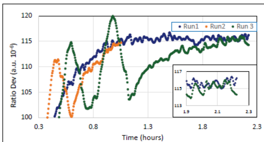
Figure 3. Three measurements of a standard 0.001\ \Omega shunt with a measurement current of 100 A. The inset is a zoomed-in view of the last 18 minutes of the measurement.
