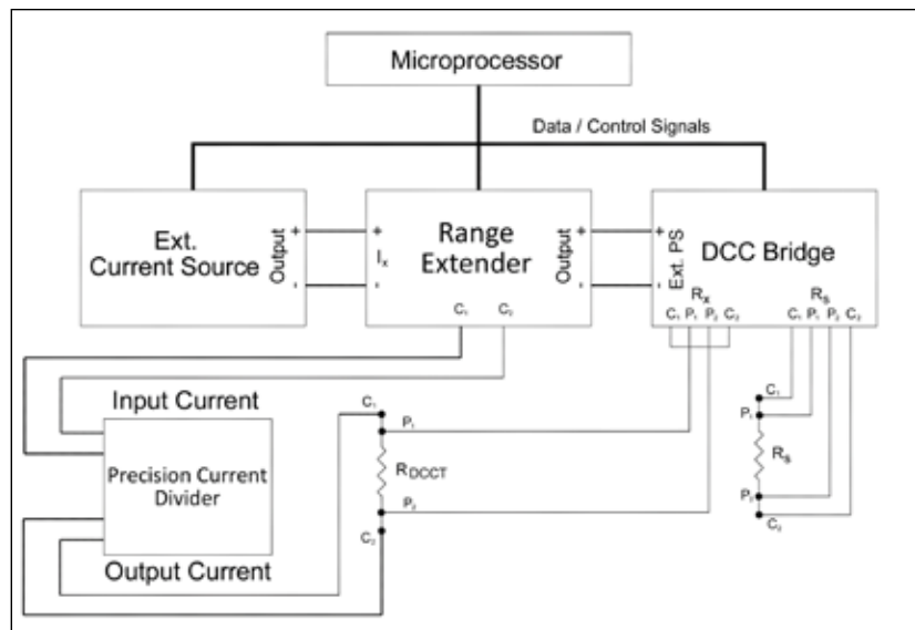
Figure 5. Block schematic of the DCCT connections to a High Current Resistance Measurement System.
